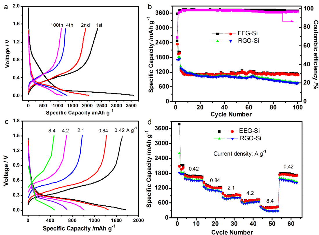
Figure 4. (a) Galvanostatic cycling profiles of EEG-Si for the first, second, fourth, and 100th cycle. (b) Cycling performance and Coulombic efficiency of EEG-Si and RGO-Si hybrids. (c) Galvanostatic cycling profiles of EEG-Si at various current densities. (d) Rate capability of EEG-Si and RGO-Si electrodes. The current densities of the three initial cycles for all of the electrodes are 105, 210, and 210 mA g -1 .
