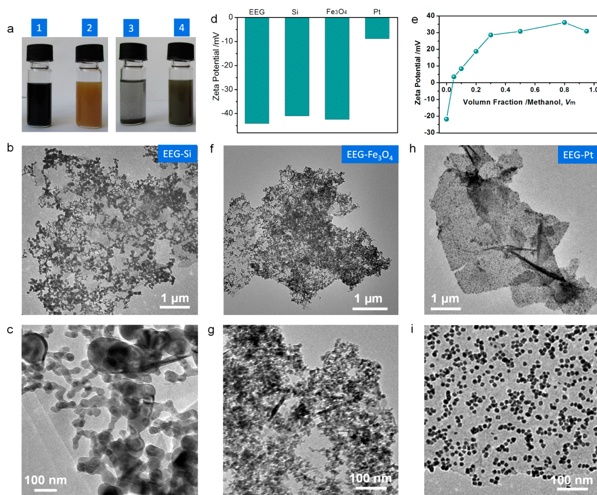
Figure 3. (a) Photographic illustration of the fabrication of EEG-Si hybrids [(1) EEG-PANB in DMF; (2) Si NPs in DMF; (3) EEG-Si obtained after mixing samples 1 and 2; (4) Suspensions of pristine EEG sheets and Si NPs]. (b) Typical TEM and (c) HR-TEM images of EEG-Si hybrids. (d) Zeta potential measurement of EEG and various colloidal nanoparticles (including Si, Fe 3 O 4 , and Pt). (e) Surface charge investigation of EEG-PANB in DMF solutions with various methanol volume fractions; (f–i) TEM and HR-TEM images of EEG-Fe 3 O 4 (f, g) and EEG-Pt hybrids (h, i).
