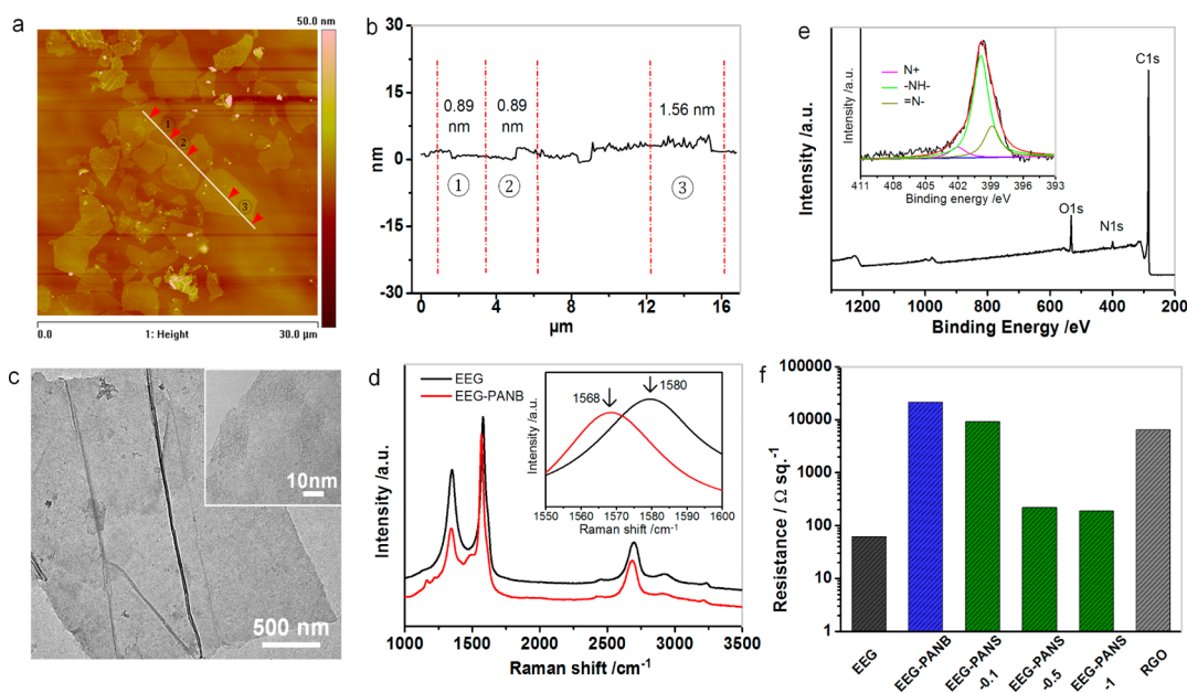
Figure 2. Characterizations of EEG and EEG-PANB. (a) AFM image of EEG sheets. (b) Height profile of EEG obtained around the white line in (a). (c) Typical TEM and HR-TEM (inset) images of EEG-PANB. (d) Raman spectra of EEG and EEG-PANB. Inset shows the shift of the G peak. (e) XPS spectra and N 1s XPS spectra (inset) of EEG-PANB. (f) Resistance comparison of EEG, RGO, and EEG-PANB before and after doping with HCl at various concentrations. The film resistance decreases with an increase in HCl concentration, indicating the increased protonation degree and electrical conductivity of EEG-PANS.
