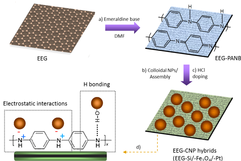
Figure 1. Synthetic procedure for EEG-CNP hybrids. (a) EEG is functionalized with emeraldine base (PANB) in DMF solutions via \pi - \pi interactions. (b) EEG-PANB sheets are assembled with a variety of colloidal nanoparticles (CNPs, e.g., Si, Fe 3 O 4 , Pt) through electrostatic interactions and hydrogen bonding. (c) Protonation of PANB with HCl gives rise to emeraldine salt (PANS) and promotes electrical conductivity of EEG hybrids. (d) Simplified cross-section view of interactions between EEG and CNPs.
